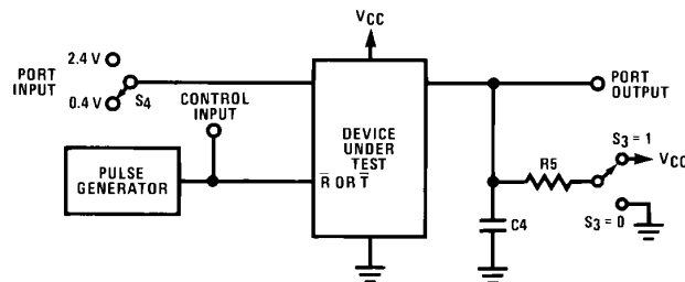
Note: C4 includes test fixture capacitance. Port input is in a fixed logical condition. See AC Table. FIGURE B. Propagation Delay to/from TRI-STATE from \bar{R} to A Port and \bar{T} to B Port
