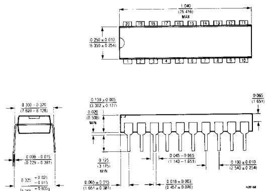
N Package 20 Lead Plastic DIP
