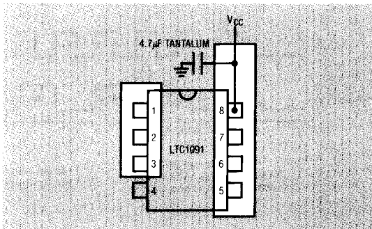
Figure 4. Example Ground Plane for the LTC1091
