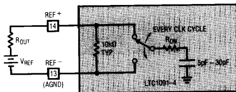
Figure 12. Reference Input Equivalent Circuit
