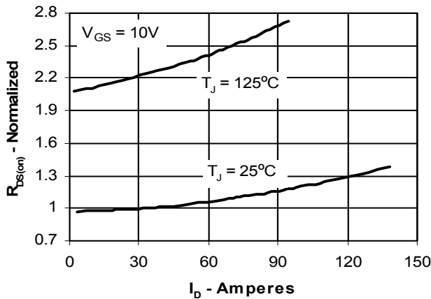
Fig. 5. R DS(on) Normalized to I D25 Value vs. I D
