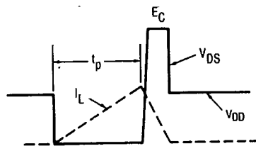
Fig. 14b — Clamped Inductive Waveforms
