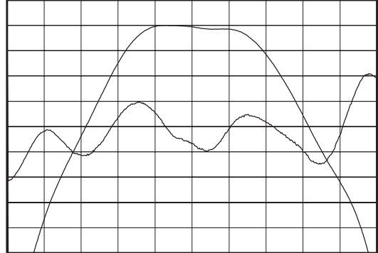
Horizontal: 300 kHz/Div Vertical: 1 dB/Div Vertical: 45 nsec/Div
