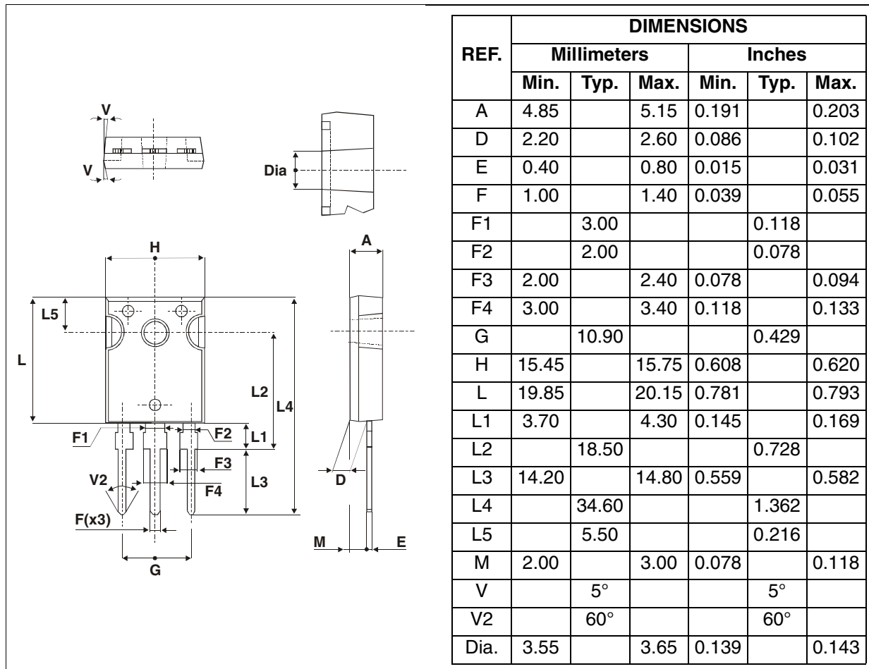
Figure 11: TO-247 Package Mechanical Data
