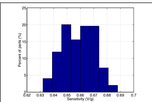
Figure 10. z-axis sensitivity at 3.3V
