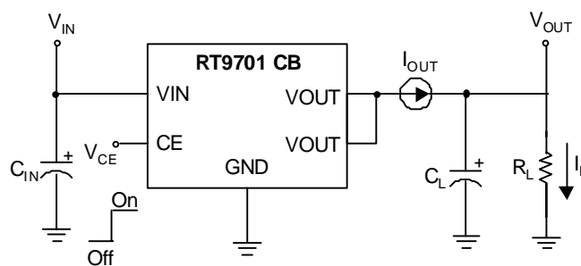
Test Circuit 3
