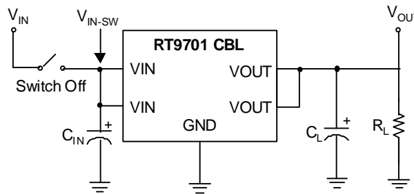
Test Circuit 2
