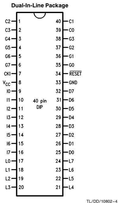
FIGURE 3. Connection Diagrams
