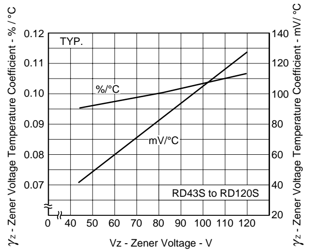
Fig. 10 ZENER VOLTAGE TEMPERATURE COEFFICIENT vs. ZENER VOLTAGE
