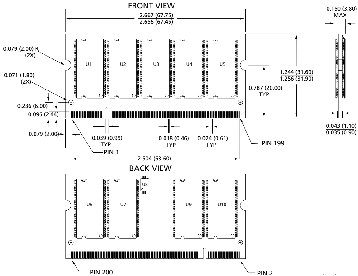
Figure 17: 200-PIN DDR SODIMM Dimensions (Low-Profile PCB)
