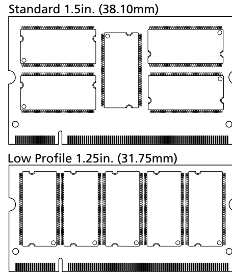
Figure 1: 200-Pin SODIMM (MO-224)
