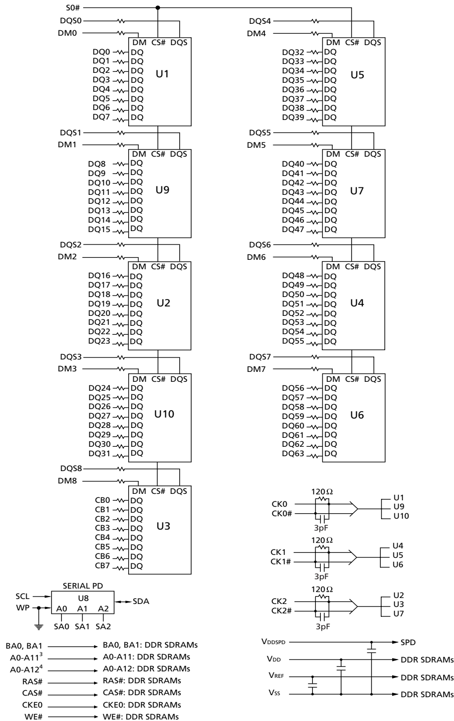
Figure 3: Functional Block Diagram, (Single-Rank, Standard Profile PCB)
