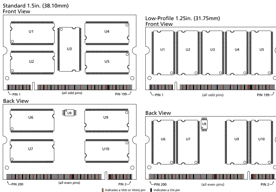
Figure 2: Module Layout
