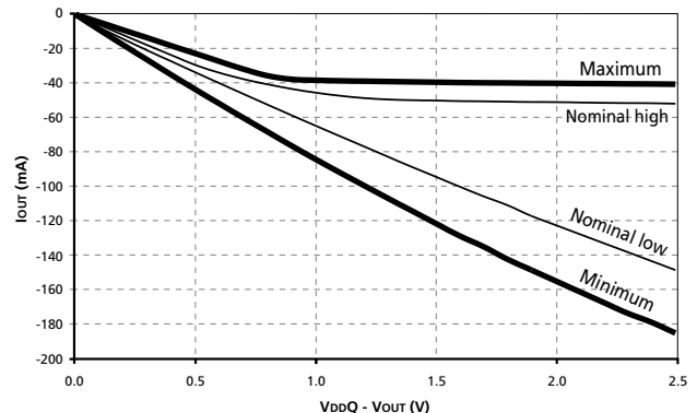
Figure 11: Pull-Up Characteristics
