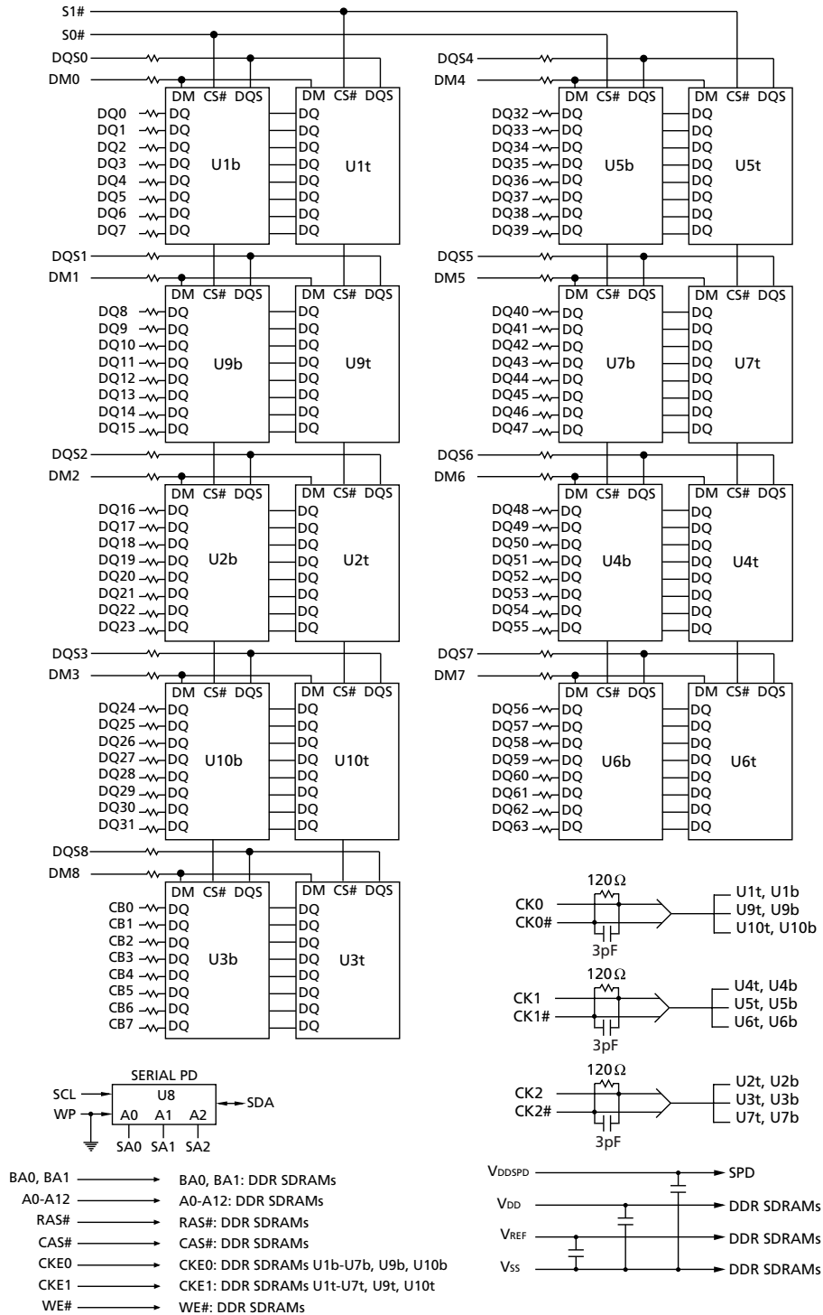
Figure 5: Functional Block Diagram, (Dual Rank, Standard Profile PCB)
