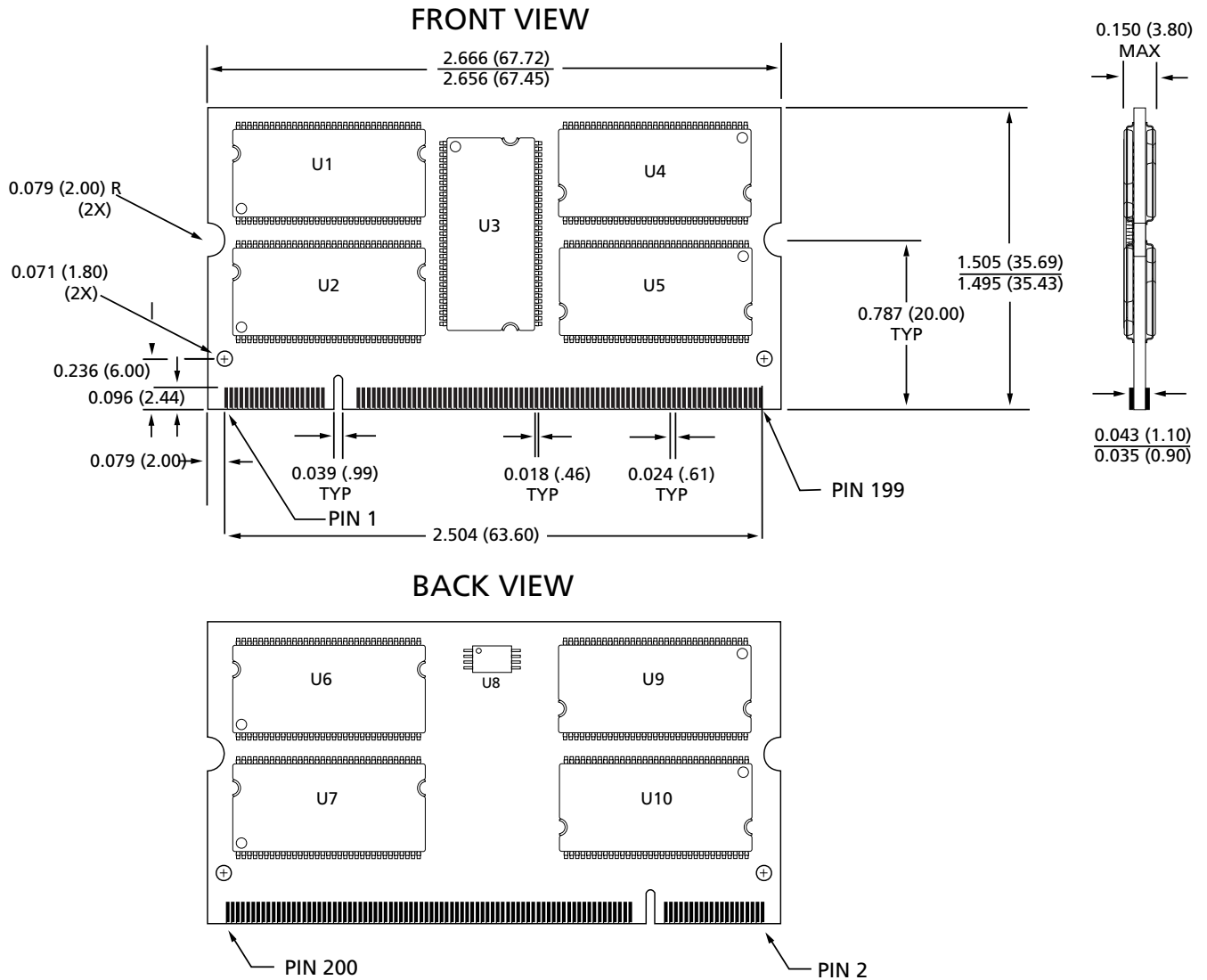
Figure 16: 200-PIN DDR SODIMM Dimensions (Standard PCB)
