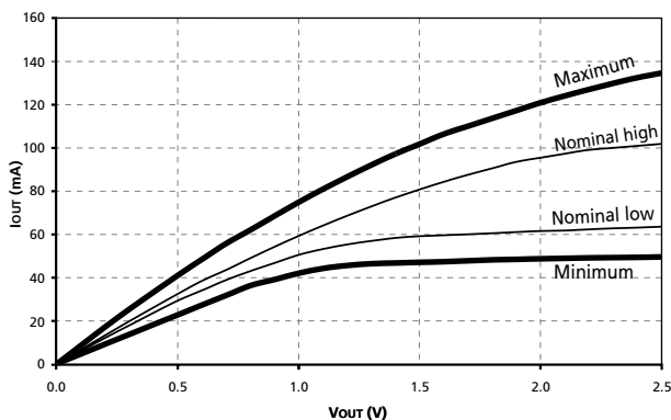
Figure 10: Pull-Down Characteristics
