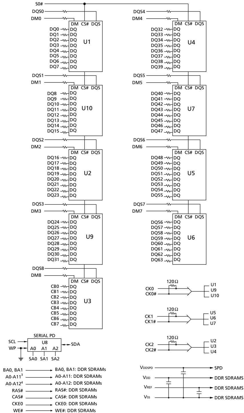
Figure 4: Functional Block Diagram, (Single Rank, Low-Profile PCB)
