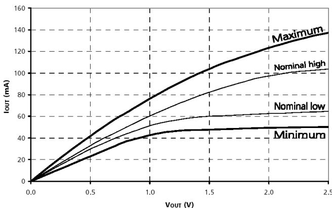
Figure 9: Pull-Down Characteristics
