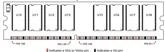
Back View -335 Speed Grade
