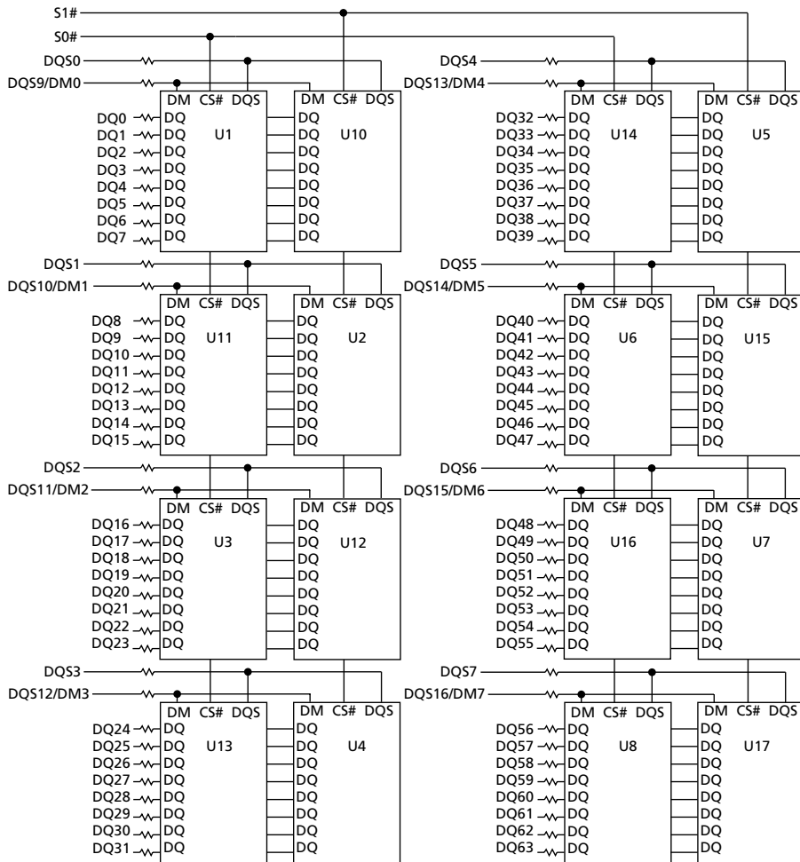
Figure 3: Functional Block Diagram -262, -26A, -265, and -202 Speed Grades
