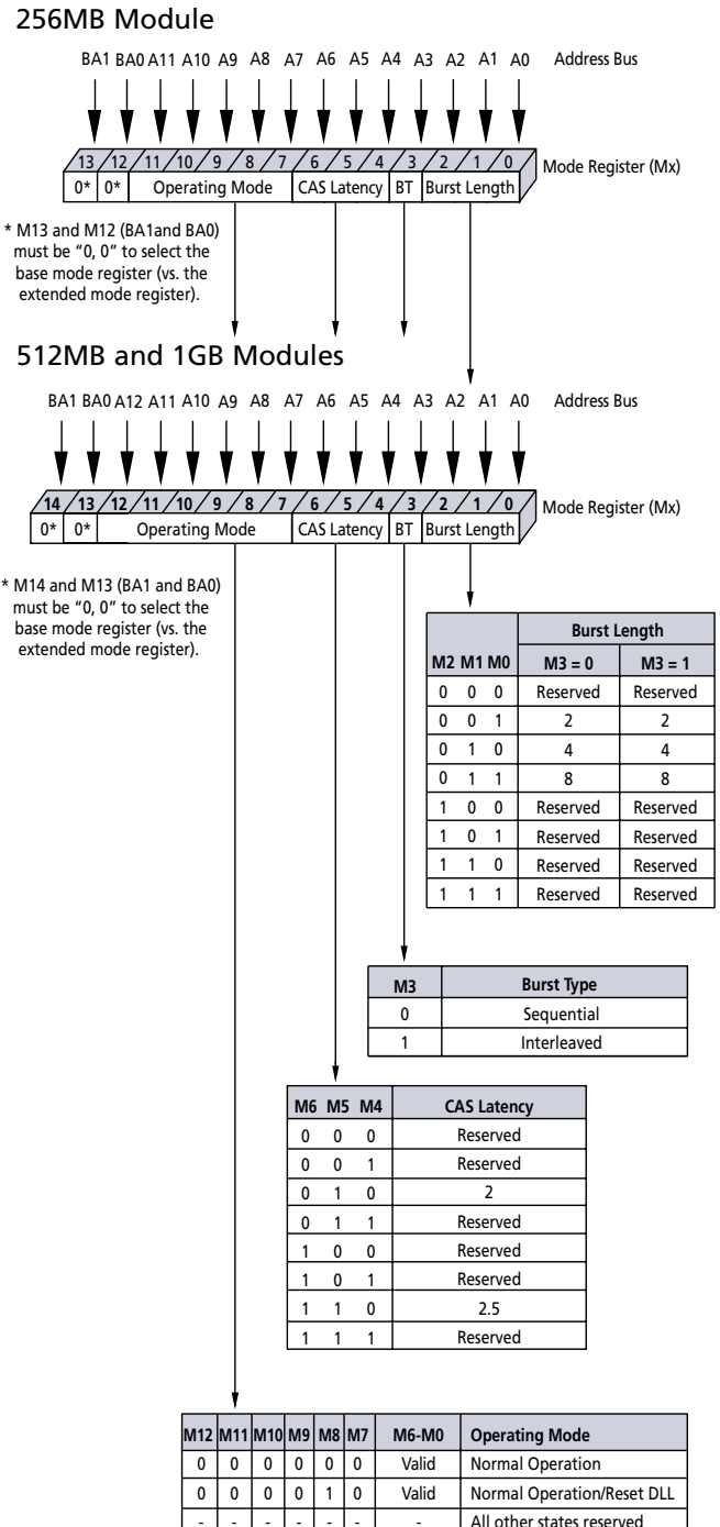
Figure 5: Mode Register Definition Diagram
