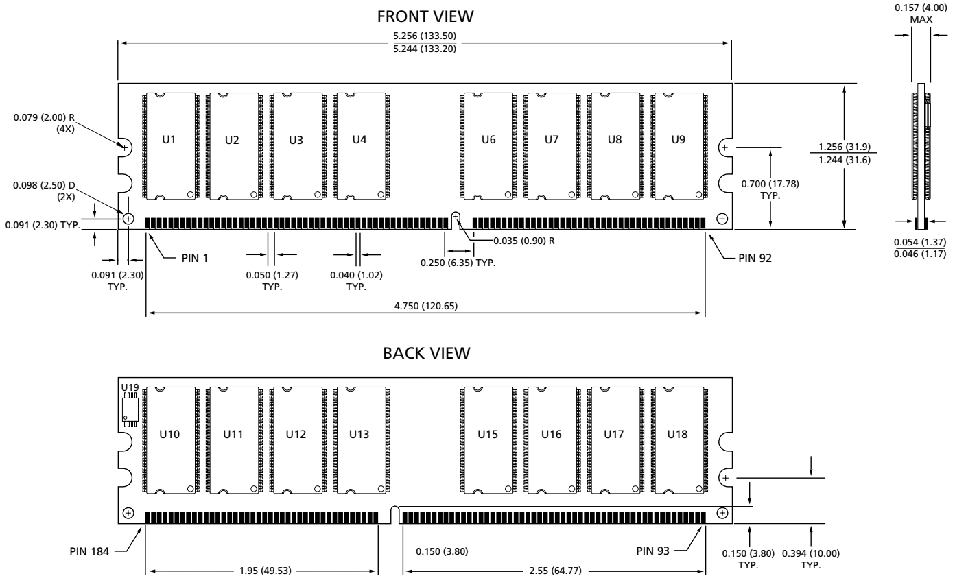
Figure 16: Standard 184-PIN DDR DIMM Dimensions, -335 Speed Grade
