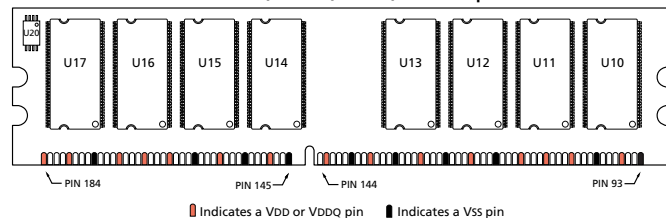
Back View -202, -265, 26A, -262 Speed Grades
