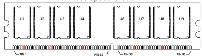
Back View -335 Speed Grade
