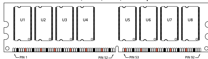
Back View -202, -265, 26A, -262 Speed Grades
