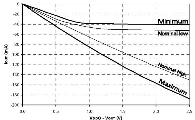
Figure 10: Pull-Up Characteristics
