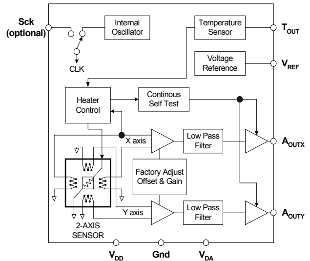
MXR2312GL/MW FUNCTIONAL BLOCK DIAGRAM
