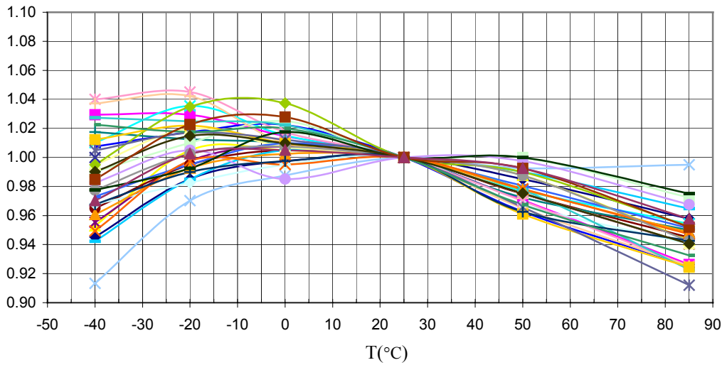
Normalized (with 25^{\circ}C ) X-axis Sensitivity vs. Temperature, V_{DD}=5V
