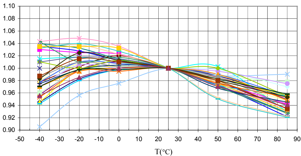
Normalized (with 25^{\circ}C ) Y-axis Sensitivity vs. Temperature, V_{DD}=5V
