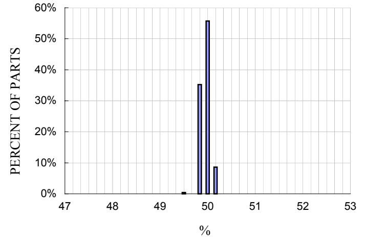
Y-axis Zero g Bias Distribution at Xout, V DD =5V
