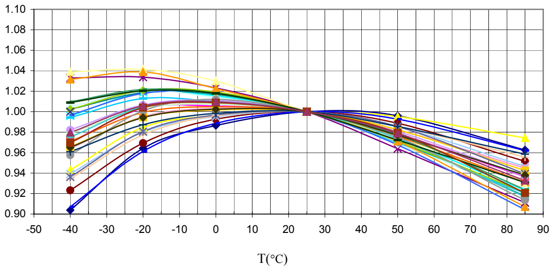
Y-axis Sensitivity Distribution at Yout, V_{DD}=3V
