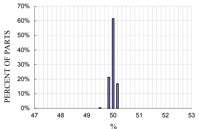
X-axis Zero g Bias Distribution at Xout, V DD =5V
