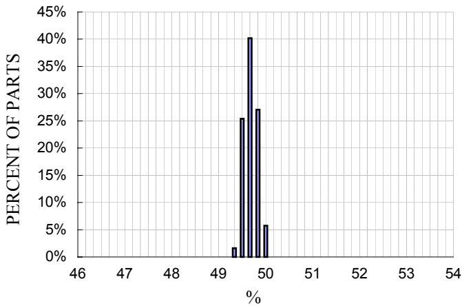
X-axis Zero g Bias Distribution at Xout, V DD =3V
