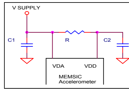
Figure 8: Power Supply Noise Rejection
