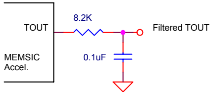
Figure 7: Temperature Output Noise Reduction
