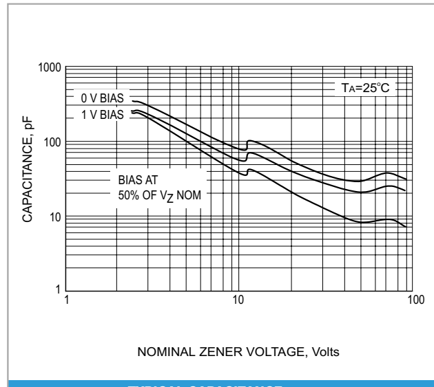
TYPICAL CAPACITANCE
