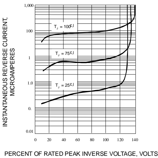
Fig. 3-TYPICAL REVERSE CHARACTERISTICS
