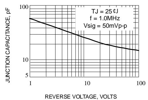
Fig. 6-TYPICAL JUNCTION CAPACITANCE
