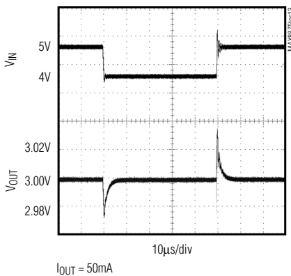
LINE-TRANSIENT RESPONSE
