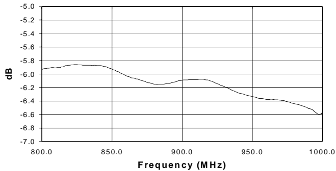
Conversion Loss
