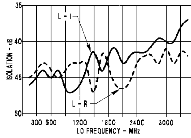
Isolation vs. Frequency
