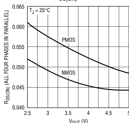
Effective R_{DS(ON)}
