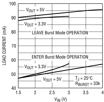
Automatic Burst Mode Thresholds vs V_{IN}
