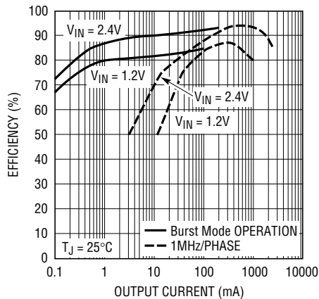
Converter Efficiency for V_{OUT} = 3.3V
