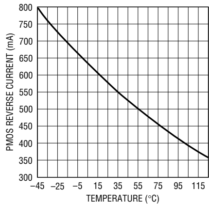
PMOS Reverse Current in Forced CCM vs Temperature
