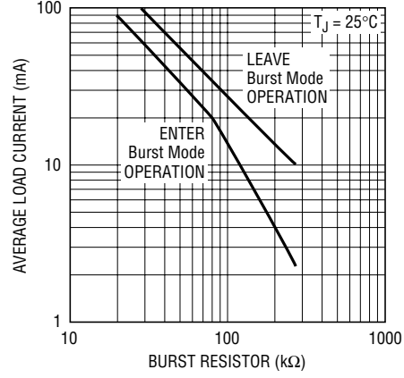
Automatic Burst Mode Current Thresholds vs R_{BURST}
