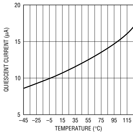
Burst Mode V OUT Quiescent Current vs Temperature
