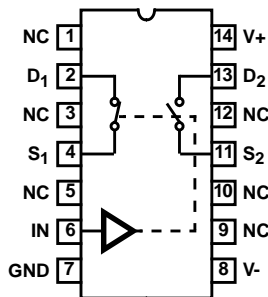
SPST HI-301 (SOIC) TOP VIEW
