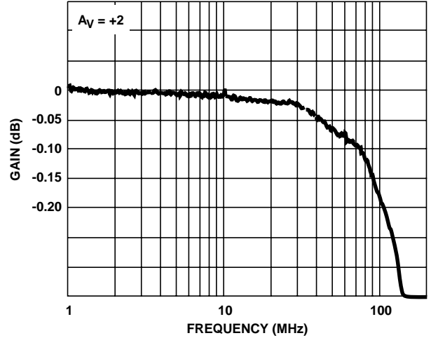
FIGURE 12. GAIN FLATNESS
