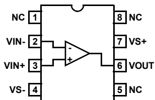
EL5111 (8-PIN HMSOP) TOP VIEW
