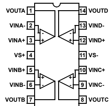
EL5411 (14-PIN HTSSOP) TOP VIEW
