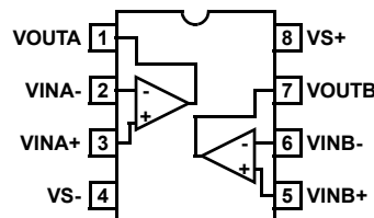
EL5211 (8-PIN HMSOP) TOP VIEW
