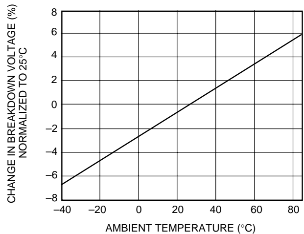
Figure 12. Switch Breakdown Voltage vs. Temperature
