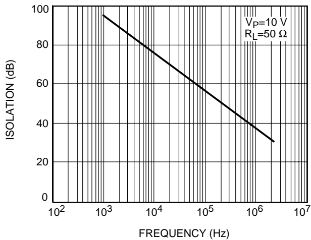
Figure 9. Output Isolation
