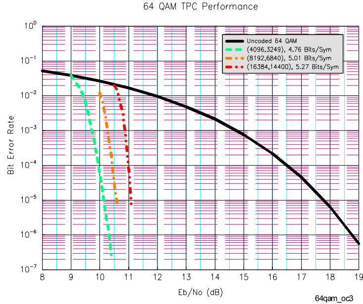
Figure 3: Performance (simulated) of Several Codes on a 64 QAM System
