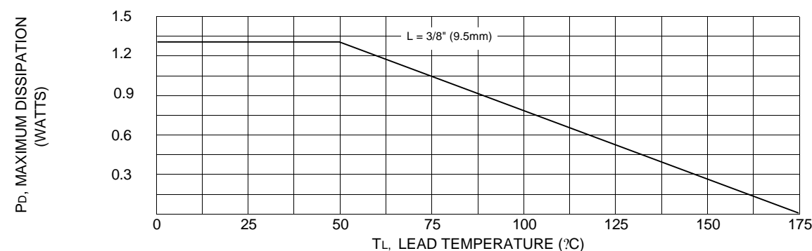
Fig. 1 POWER TEMPERATURE DERATING CURVE
