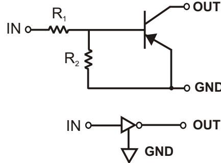
SCHEMATIC DIAGRAM
