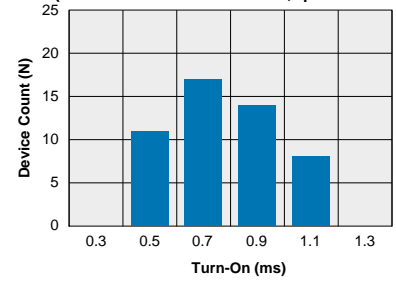
LCA127 Typical Turn-On Time (N=50 Ambient Temperature = 25°C) (Load Current = 170mADC; I_F = 5\text{mADC} )
