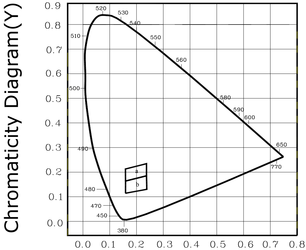
Chromaticity Diagram(Y)
