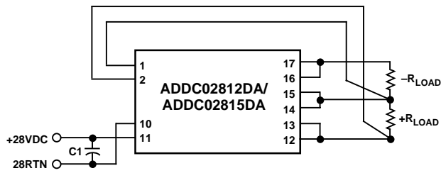
NOTE: VALUE OF C1 IS DEPENDENT ON SOURCE IMPEDANCE. REFER TO SECTION ON SYSTEM INSTABILITY CONSIDERATIONS.
