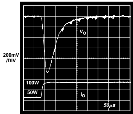
Figure 8. Output Voltage Transient Response to a 50% to a 100% Step Change in Load with Zero Load Capacitance (ADCC02815DA)
